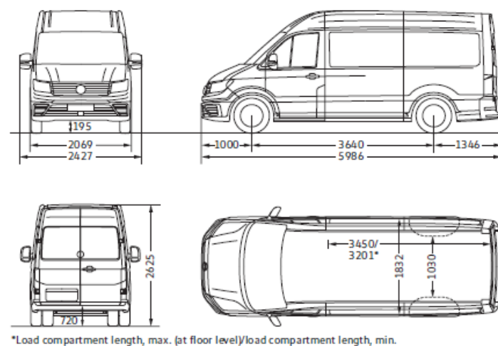
Crafter 50/55 Delivery Van medium wheelbase with high roof
