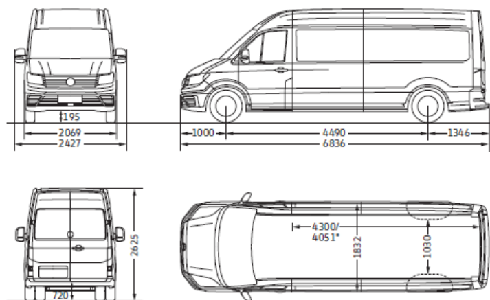
Crafter 50/55 Delivery Van long wheelbase with high roof
