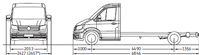
Crafter 35 Chassis long wheelbase with single cab
